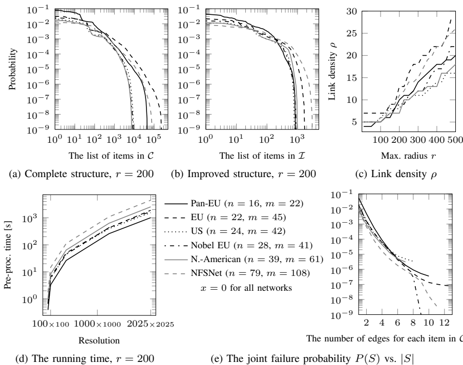
Fig. 6. The space and time complexity of the data structures for the examined network topologies.
