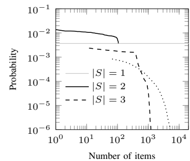
Fig. 8. The probabilities of the items in \mathcal{C} for NFSNet and r = 200 km.
