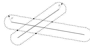
Fig. 4. The arrangement of hippodromes for two lines. The dots are the vertices and the dashed lines are the arcs.
