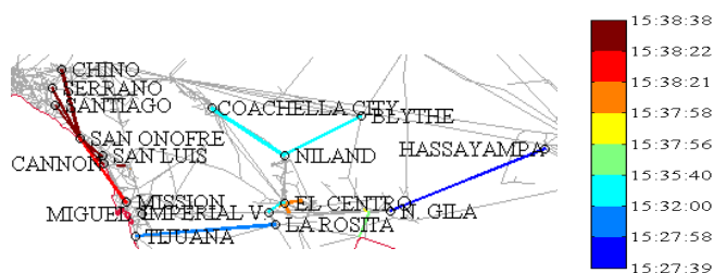
Fig. 1. The development of the Sept. 8, 2011 San Diego blackout according to [11] (the color of each line represents the time in which it tripped). The cascade development is not contiguous.
